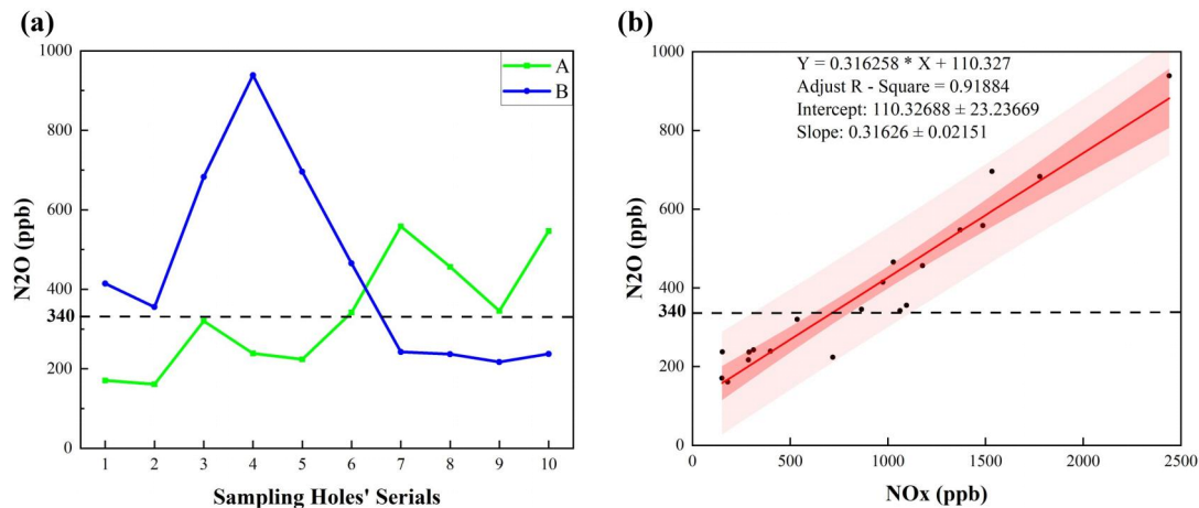
Figure 3 Flue Gas Sample Test Results. (a) \text{N}_2\text{O} Concentrations in Flue Gas From Different Sampling Holes
