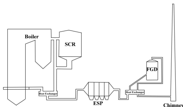
Figure 1 Flowchart of Ultra-Low Emission Technology in Coal-Fired Power Plants
